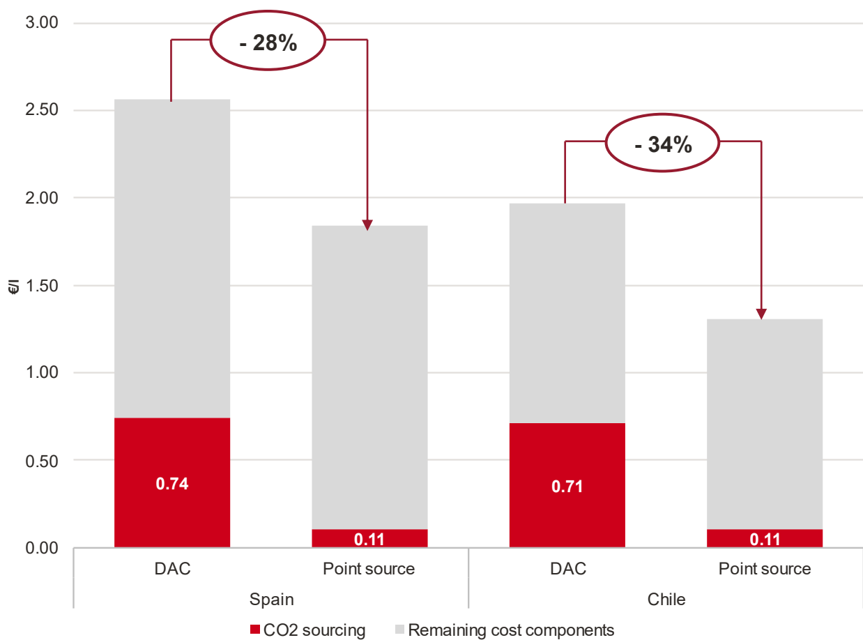
Figure 19 E-fuels production costs with different CO 2 sources
