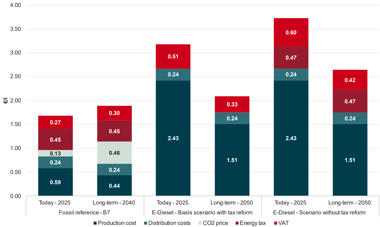
Figure 21 Price components of e-diesel and fossil diesel (B7), averages of the bandwidths in 2025 and in the long term
