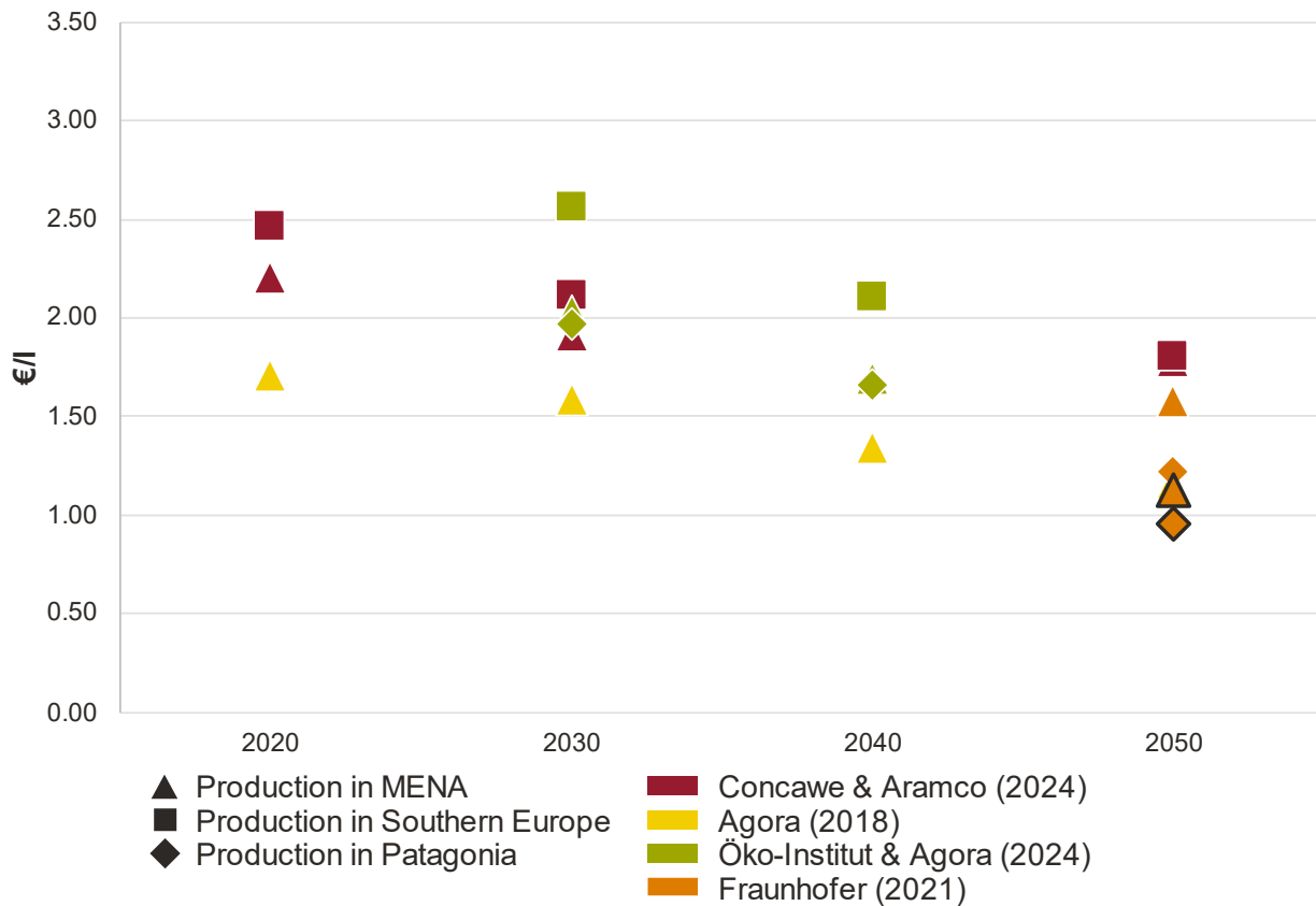
Figure 4 Literature review: Production costs (incl. transport) of e-diesel in 2020, 2030, 2040 and 2050
