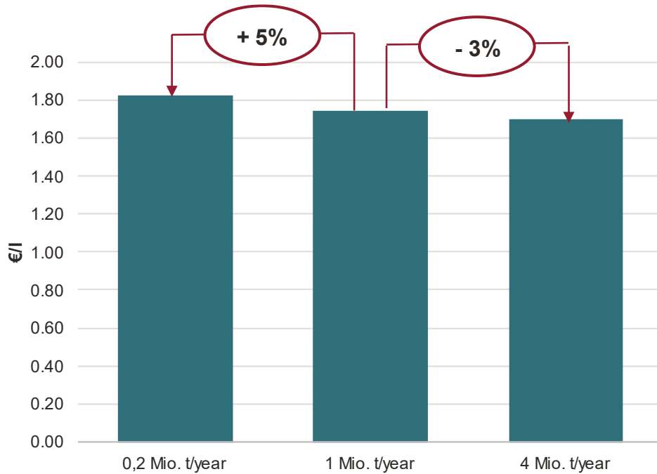
Figure 20 E-fuels production costs by production capacity
