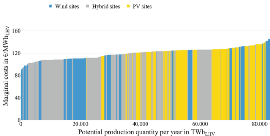
Figure 5 Marginal costs and production potential for Fischer-Tropsch diesel in 2050
