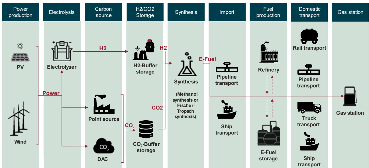
Figure 2 The e-fuels value chain
