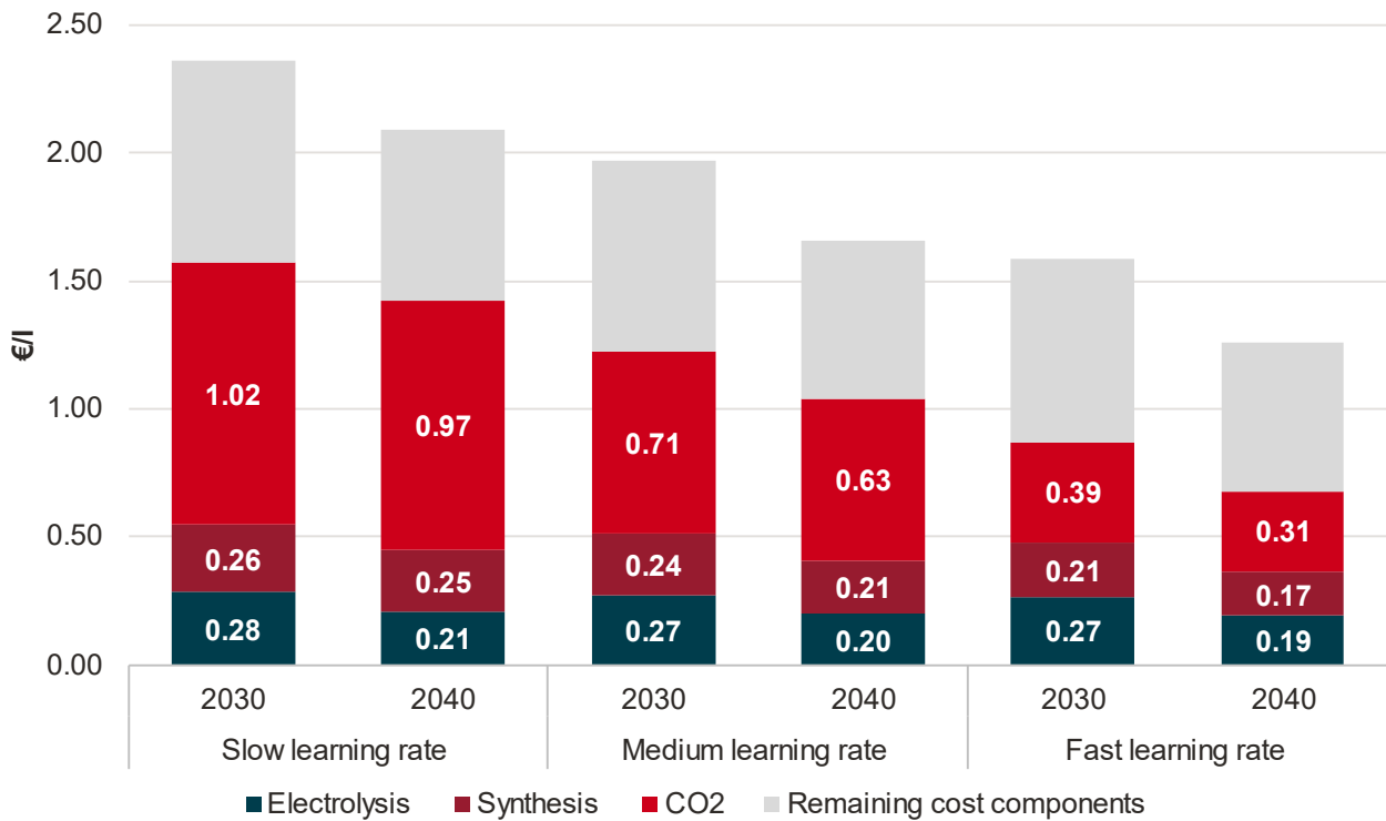
Figure 7 E-fuels production costs with different learning rates
