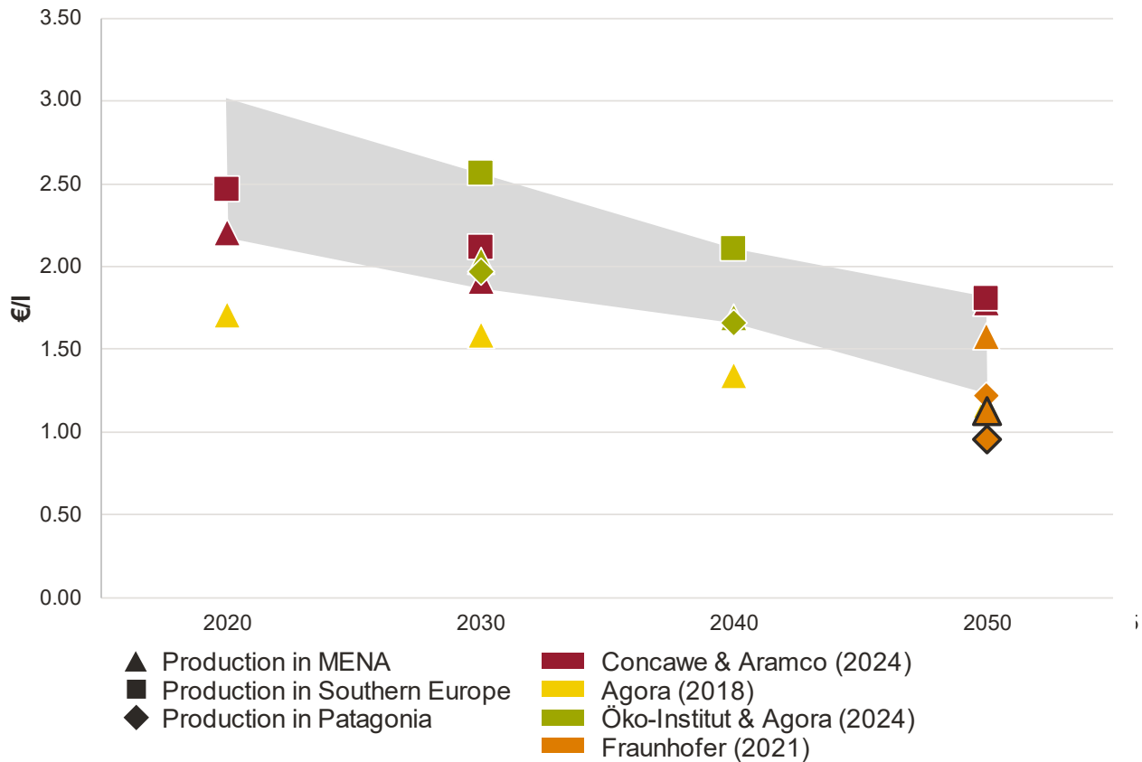
Figure 8 Literature review: Production costs of e-diesel incl. transport, 2020-2050, and resulting range
